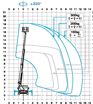
WORKING ENVELOPE
