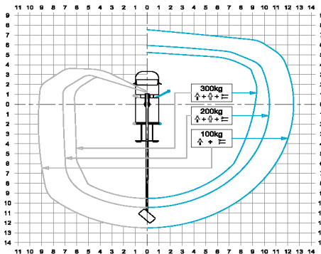
OUTRIGGER FOOTPRINT
